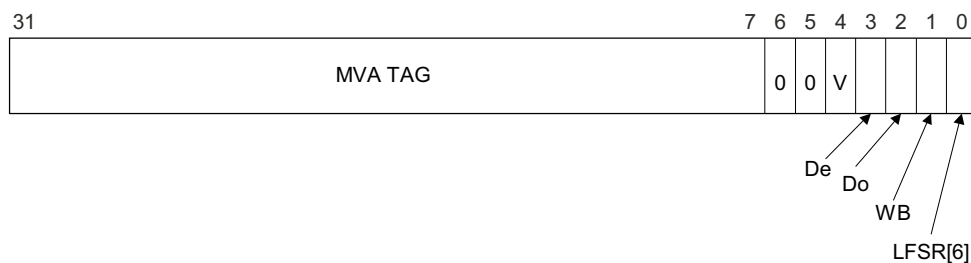
Figure 11-7 Data format, CAM read
